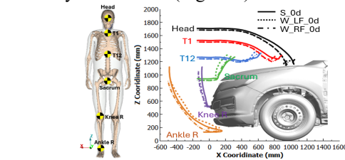
Figure 4. Trajectories from three gaits in a lateral impact
