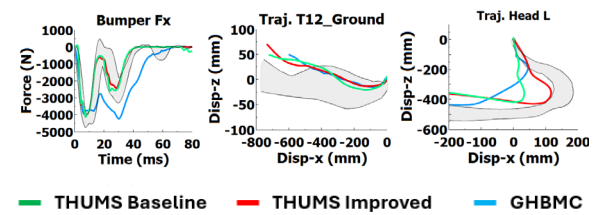
Figure 3. Bumper force, T12 and head trajectory compared
