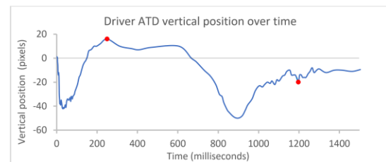
Figure 4: Vertical motion tracking of the Driver ATD head. Red dot 1: Vertical peak of the ATD head motion. Red dot 2: Helmeted ATD head-strike against the vehicle side wall.
