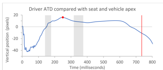
Figure 5: Vertical tracking of the Driver ATD head from the start of the blast to the beginning of vehicle ground impact (red line); the shaded areas represent the peaks of vertical motion – firstly the seat, and then the vehicle.
