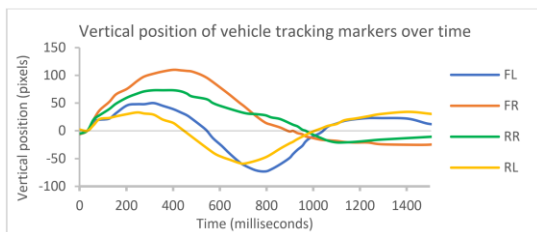
Figure 3: Vertical motion tracking using the pole tracking markers positioned on all four corners of the vehicle – Front Left (FL), Front Right (FR), Rear Right (RR), Rear Left (RL).
